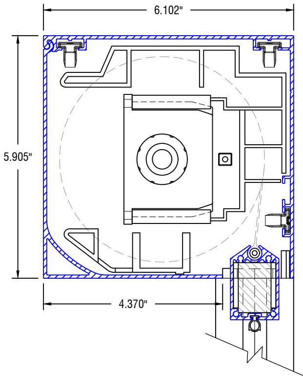
IDLER PROFILE
