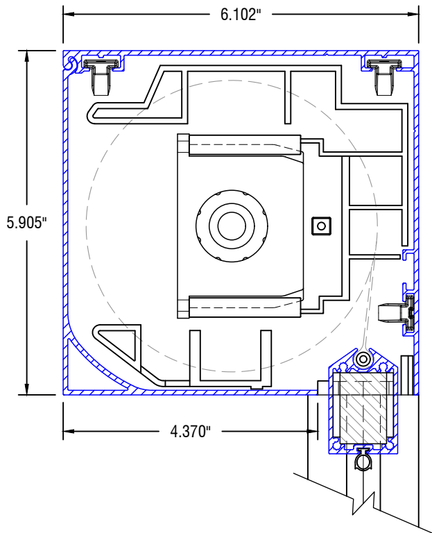
IDLER PROFILE
