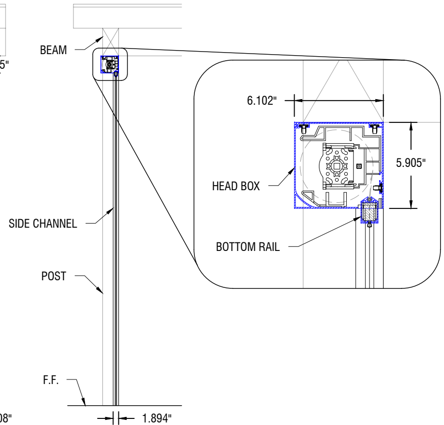
2 PATIO SECTION
