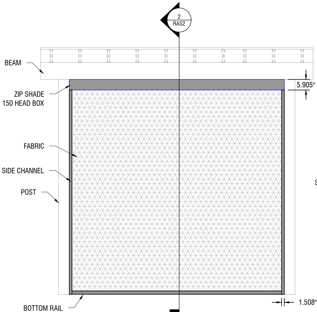
1 EXTERIOR PATIO ELEVATION
