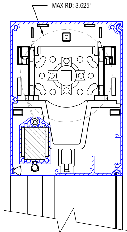
MOTOR PROFILE
