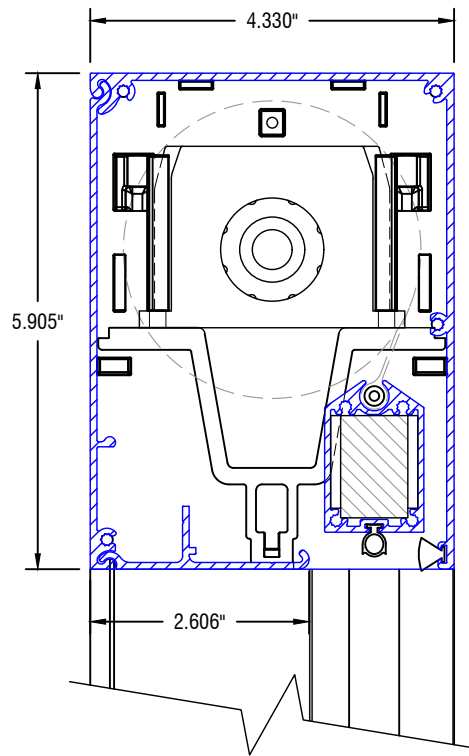
IDLER PROFILE
