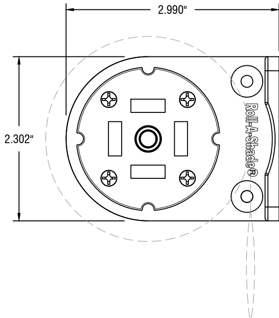
IDLER PROFILE
