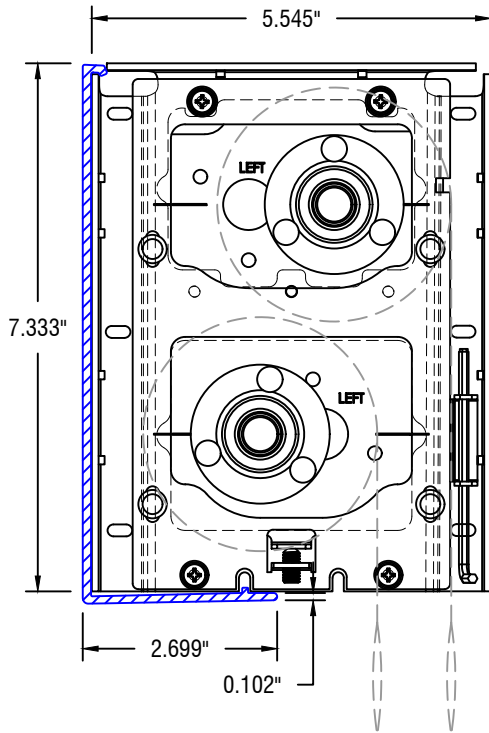
IDLER PROFILE
