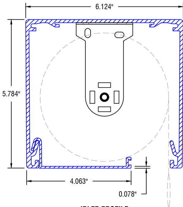
IDLER PROFILE
