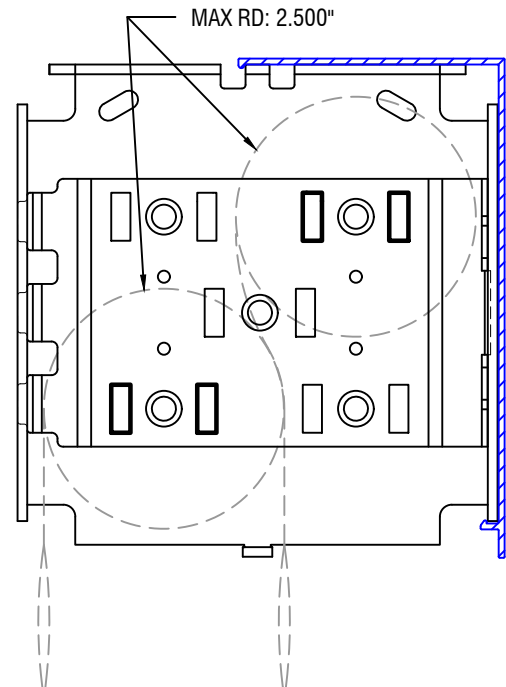
CLUTCH PROFILE
