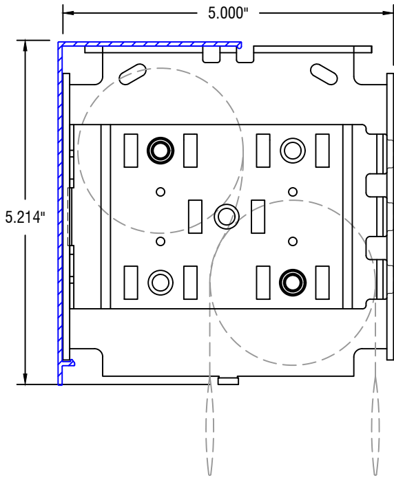
IDLER PROFILE
