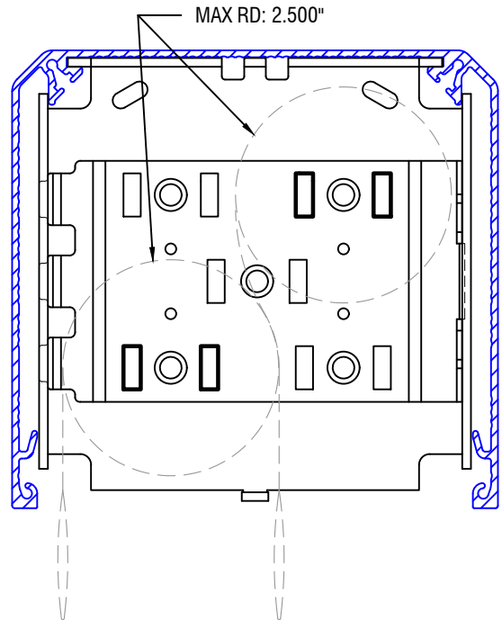
CLUTCH PROFILE
