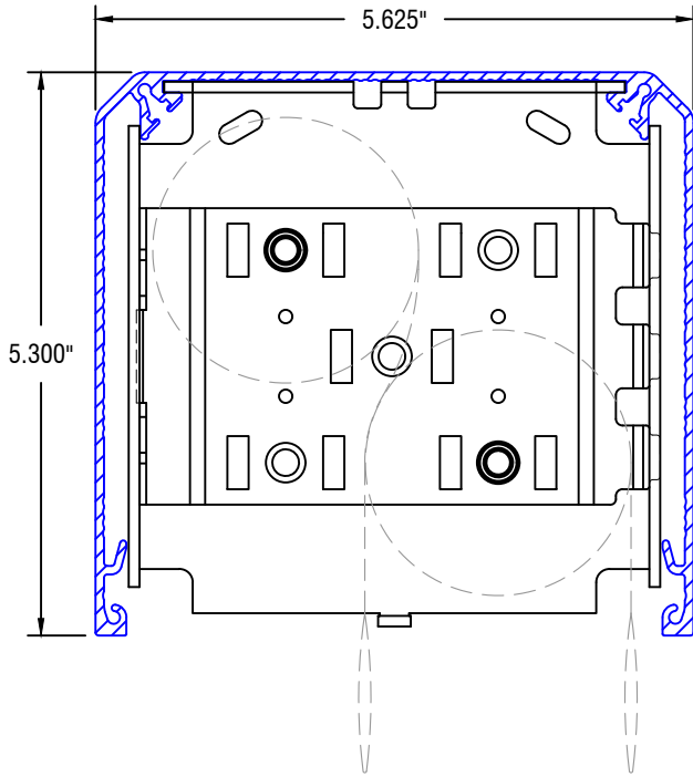
IDLER PROFILE
