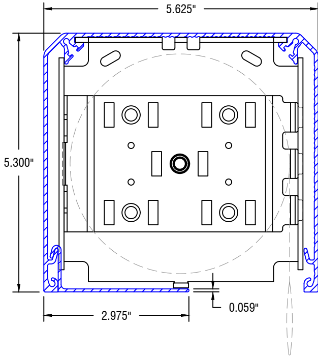
IDLER PROFILE
