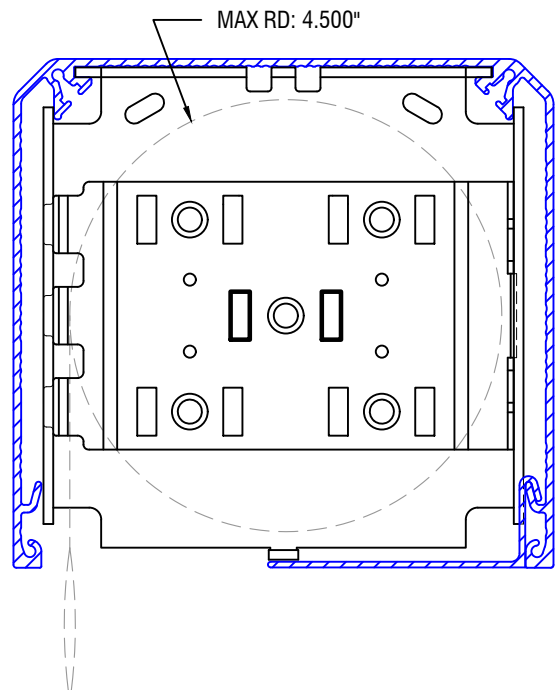
CLUTCH PROFILE
