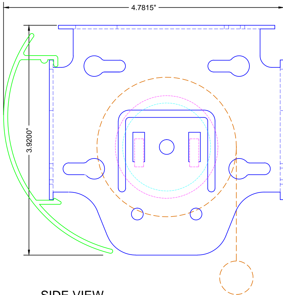
SIDE VIEW
