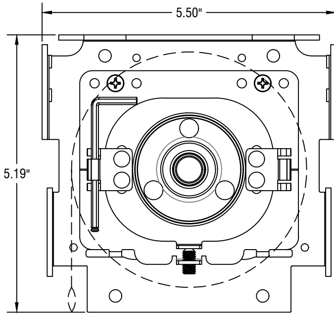
FRONT VIEW - IDLER
