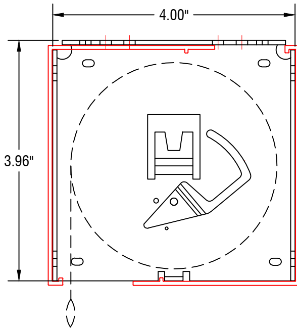
FRONT VIEW - IDLER
